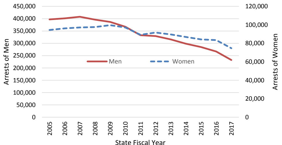
Figure 1: Total Arrests in Illinois, by Gender
